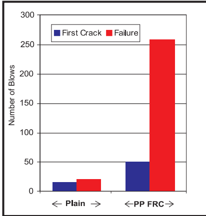
IMPACT STRENGTH (FRC 14 times greater than plain Concrete)
