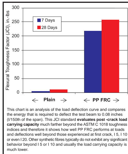
FLEXURAL TOUGHNESS FACTOR
