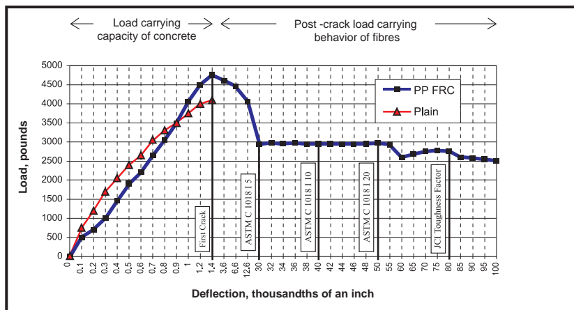
LOAD DEFLECTION CURVE
