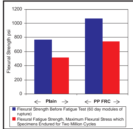
FLEXURAL FATIGUE STRENGTH (FRC Fatigue Strength/Endurance 30% greater than plain Concrete)
